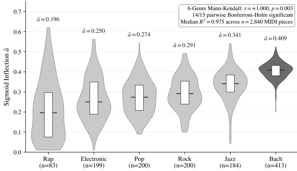
Figure 6: Genre hierarchy across six macro-genres: Rap ( \tilde{a} = 0.196 ) → Electronic → Pop → Rock → Jazz → Bach (Classical, \tilde{a} = 0.409 ); Mann-Kendall \tau = +1.000 , p = 0.003 . n = 2,840 MIDI pieces.
