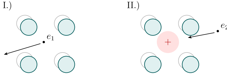
Figure 2: The lattice distortion caused by e_1 (I.) outlives its passage and attracts a second electron e_2 (II.).
