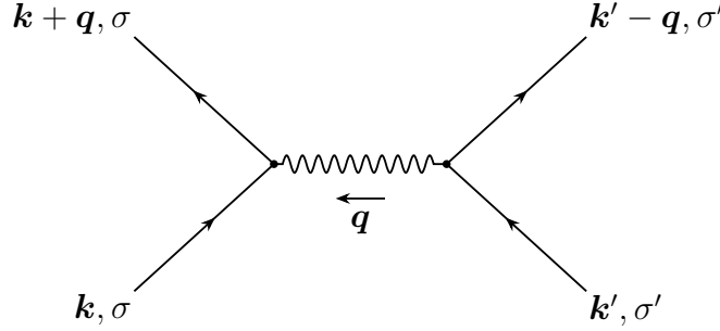
Figure 3: Vertex corresponding to eq. (42): two electrons exchange a phonon of momentum \mathbf{q} .
