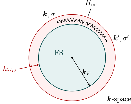
Figure 4: Only states in a shell of width \hbar\omega_D around the Fermi surface take part in the effective interaction.
