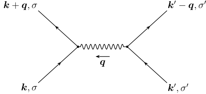
Figure 2: Vertex corresponding to eq. (2): two electrons exchange a phonon of momentum \mathbf{q} .
