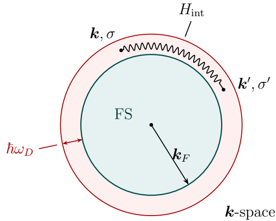
Figure 3: Only states in a shell of width \hbar\omega_D around the Fermi surface take part in the effective interaction.
