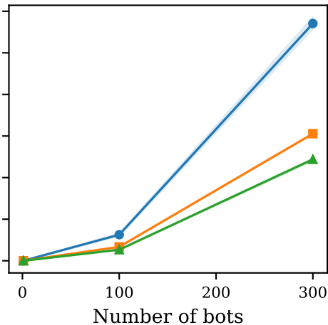
Regional (900-1000 ms)
