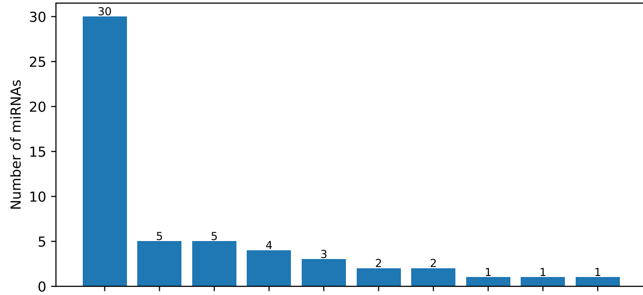
C Disease-category overlap
