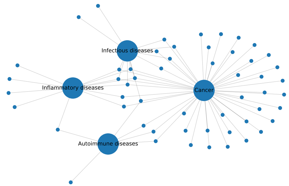
B miRNA-disease-category network
