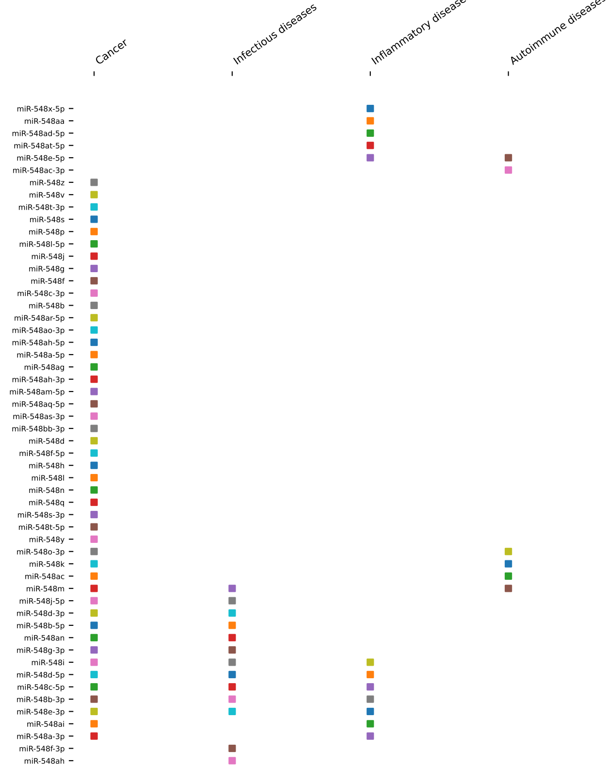
A Disease-profile matrix ordered by Jaccard/average-linkage clustering Figure 7. Disease-association architecture of the miR-548 family
