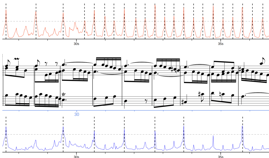
Figure 5.3: LayerIt activation-and-position display for BWV 856. The upper panel shows BeatThis beat logits and selected beat estimates; the time-warped score occupies the middle panel; and the lower panel shows downbeat logits and estimated downbeat positions.
