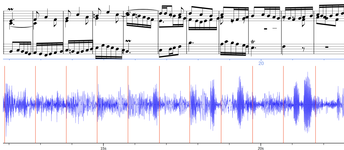
Figure 5.4: LayerIt waveform display an excerpt for BWV 856 by András Schiff, with BeatThis beat positions aligned to the time-warped score.
