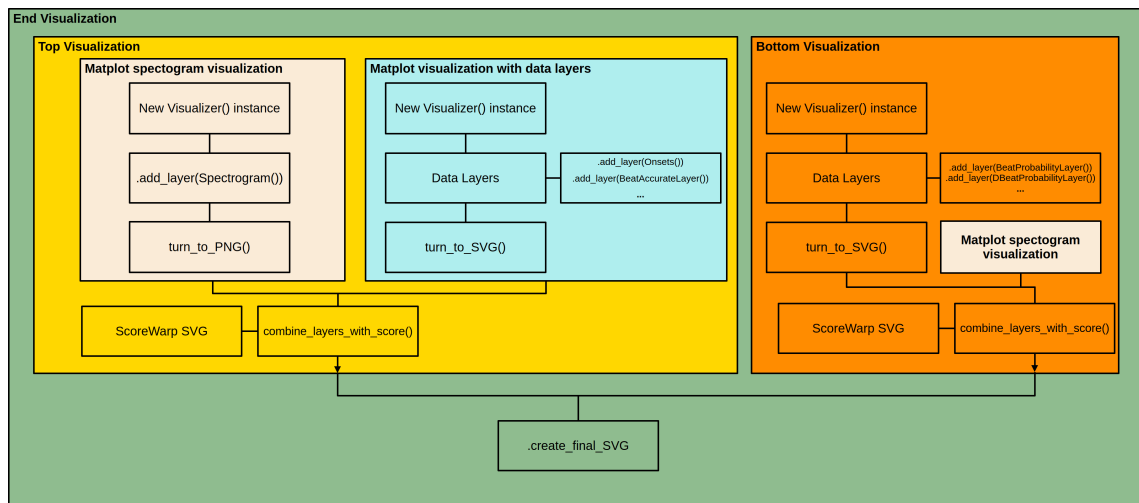
Figure 4.3: Simplified Block Diagram for generating Figure 4.2. Demonstrating the different levels for generating the combined aligned visuals, colored boxes show different levels of visualizations. Note that the beige boxes labeled "Matplot spectrogram visualization" refers to the same PNG element that is being called within the same script that is generating the whole visualization.
