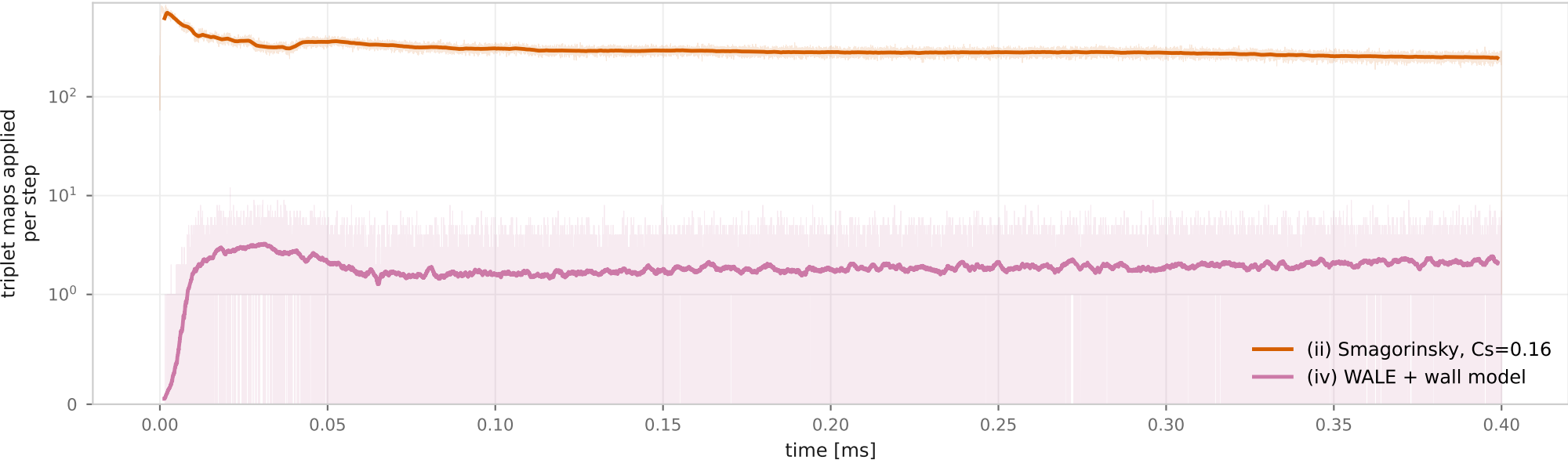
(b) eddy events actually mapped onto the LEM line
