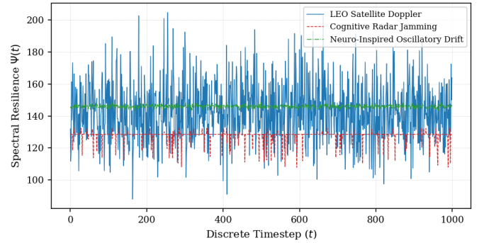
Fig. 2. Dynamic Spectral Resilience Function \Psi(t) across three CAMAE scenarios. Radar jamming events produce sharp transients with rapid recovery within 1–2 timesteps.
