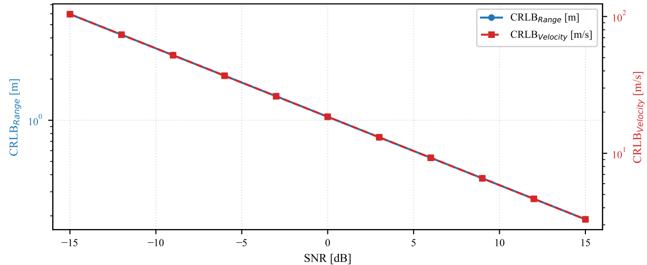
Cram'er-Rao Lower Bound for ISAC Estimation
