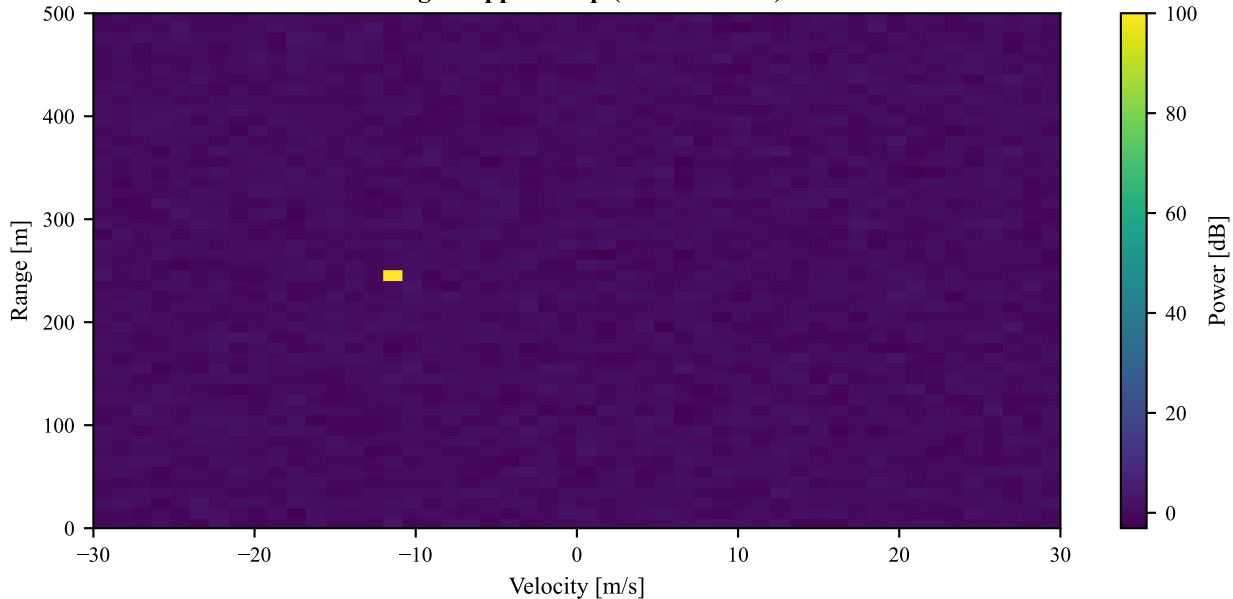
Range-Doppler Map (OFDM-ISAC)
