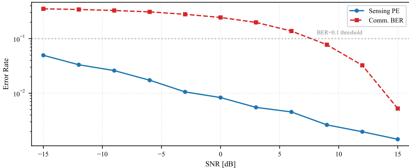
ISAC Joint Performance: Sensing vs Communication
