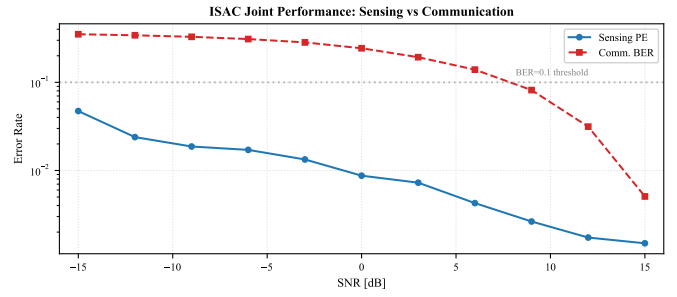
Fig. 1: Joint sensing and communication performance: sensing prediction error (PE) and communication bit error rate (BER) as functions of SNR. The 10^{-1} BER threshold is indicated for reference.
