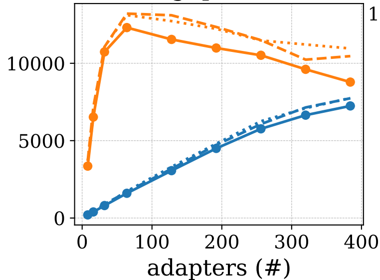
Throughput (toks/s)
