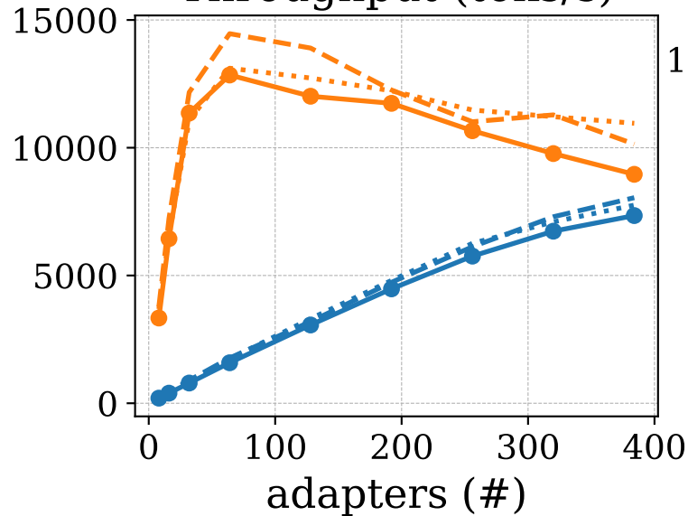
Throughput (toks/s)
