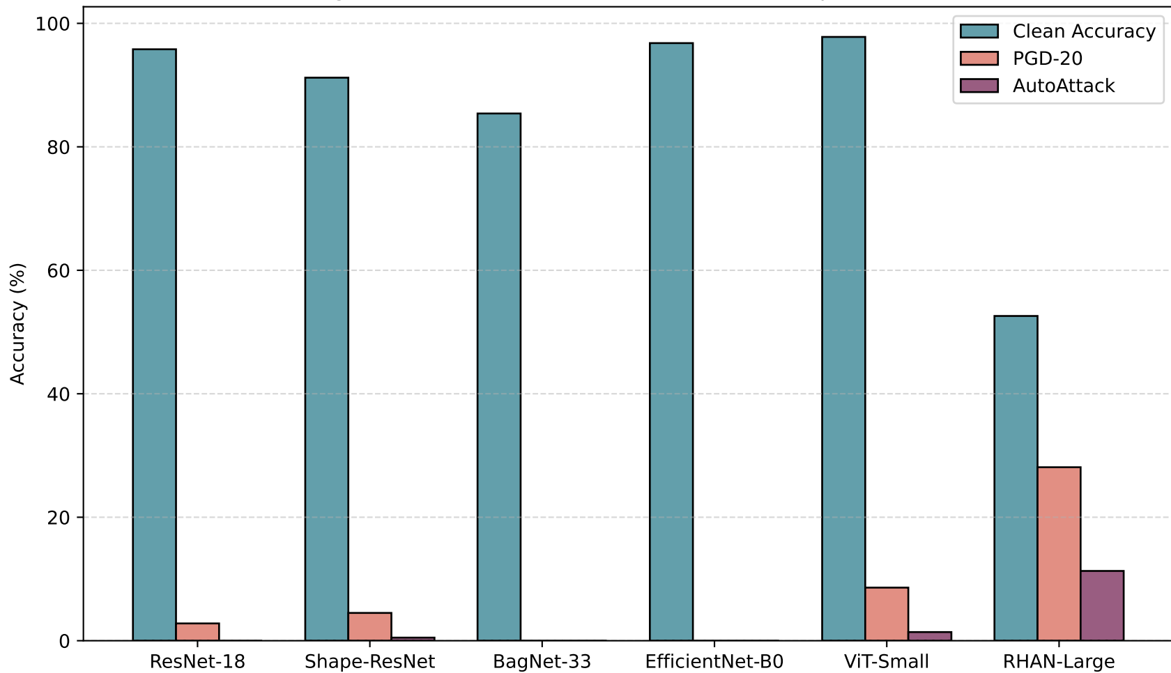
Figure 1: Classical Architectures (Our Own Experiments)
