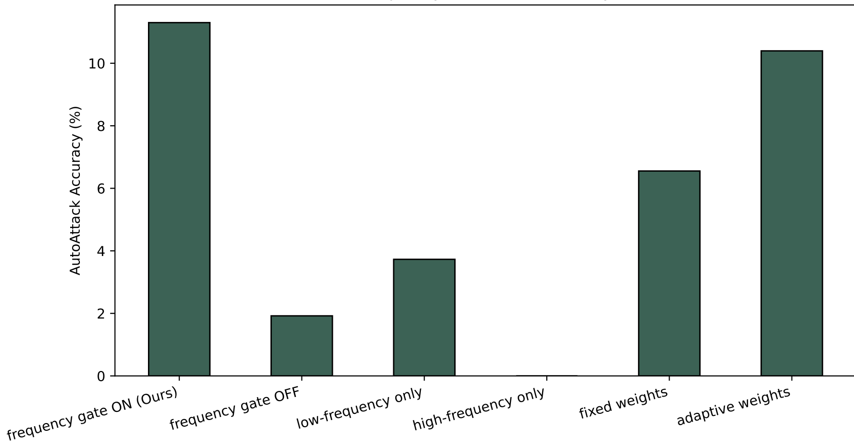
Frequency Gate Ablation Study
