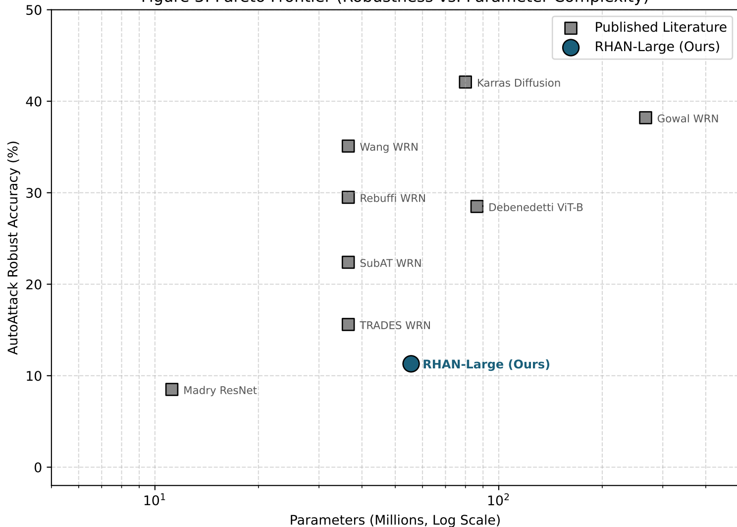
Figure 3: Pareto Frontier (Robustness vs. Parameter Complexity)
