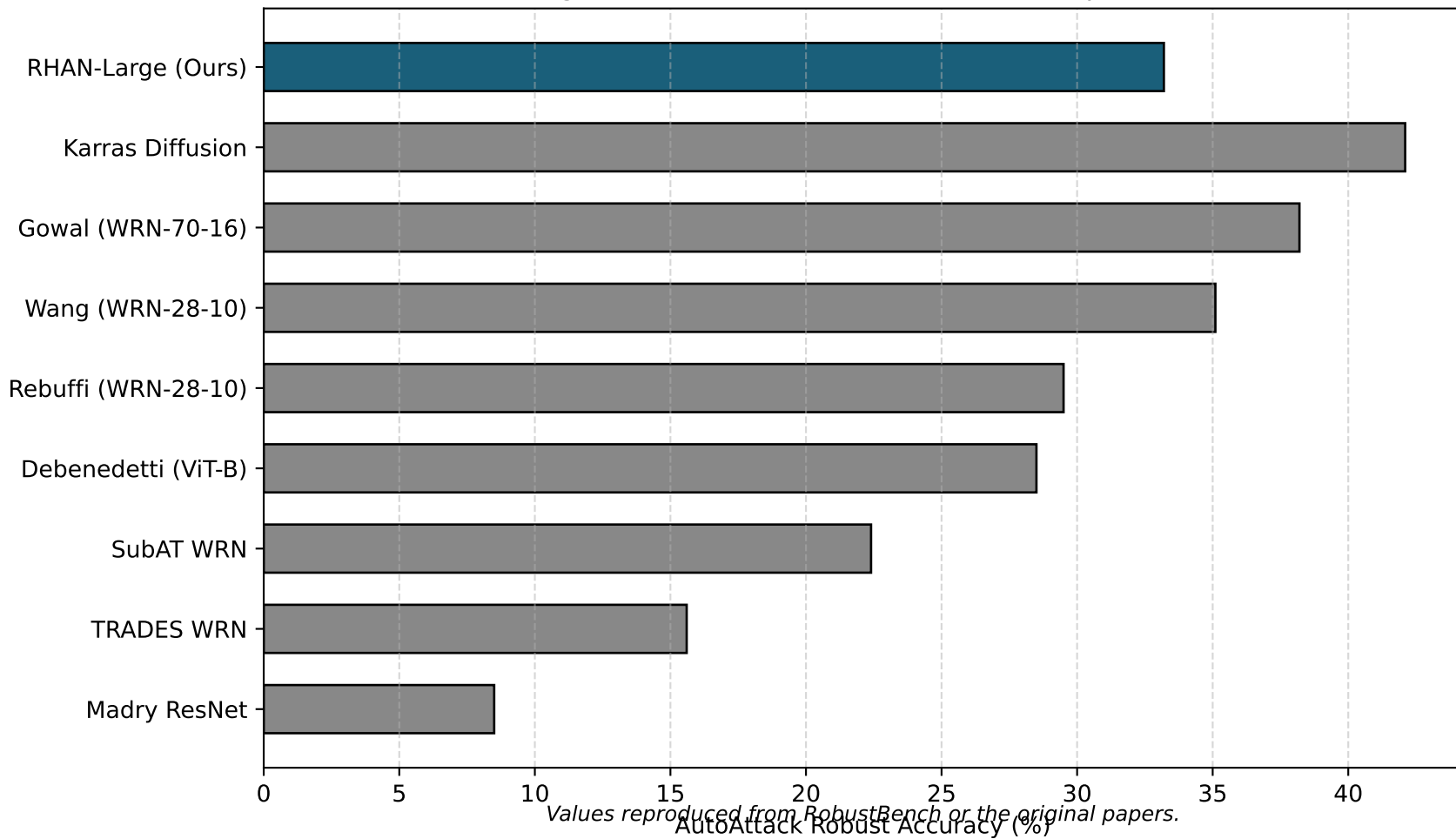
Figure 2: RobustBench / Literature Comparison
