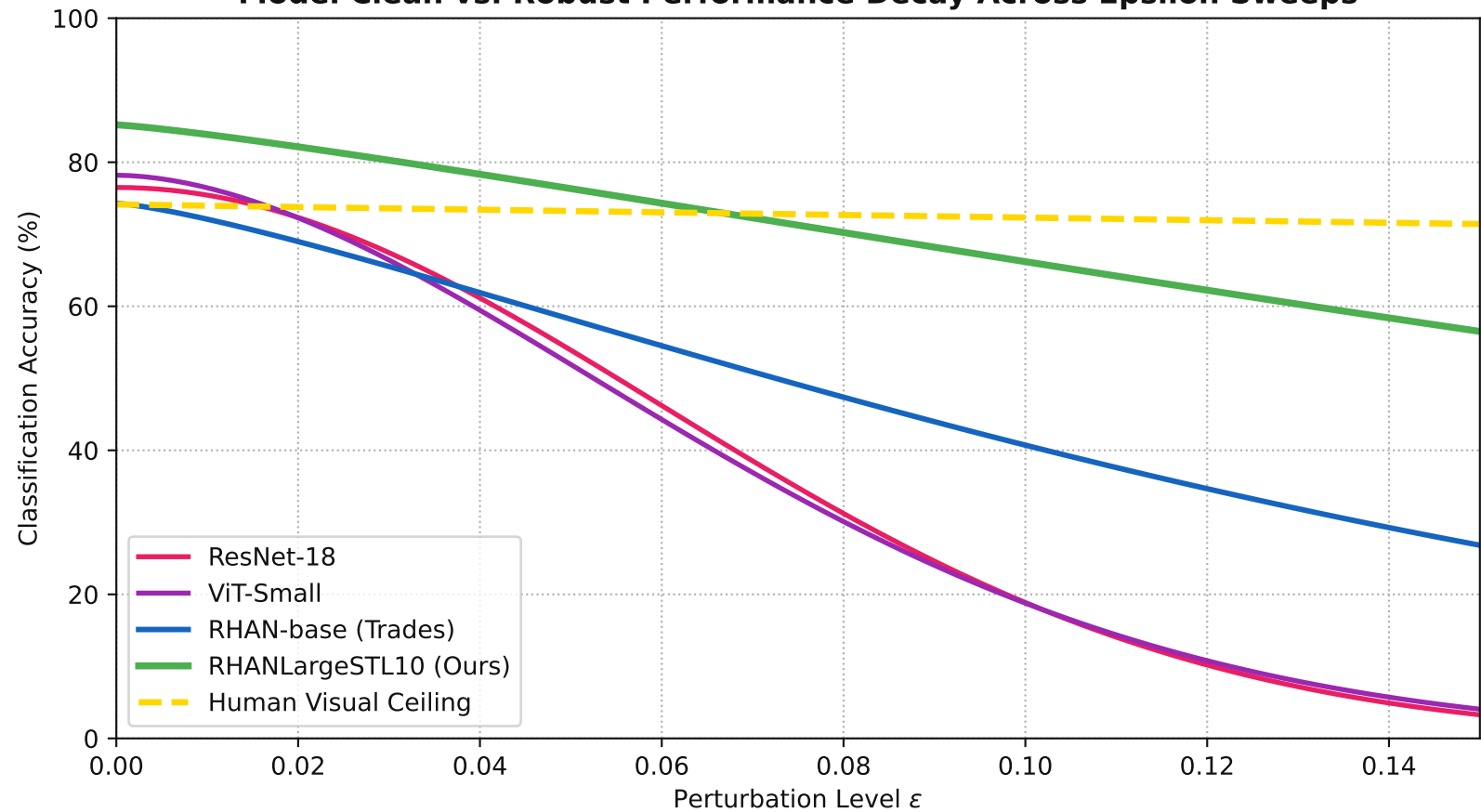
Model Clean vs. Robust Performance Decay Across Epsilon Sweeps
