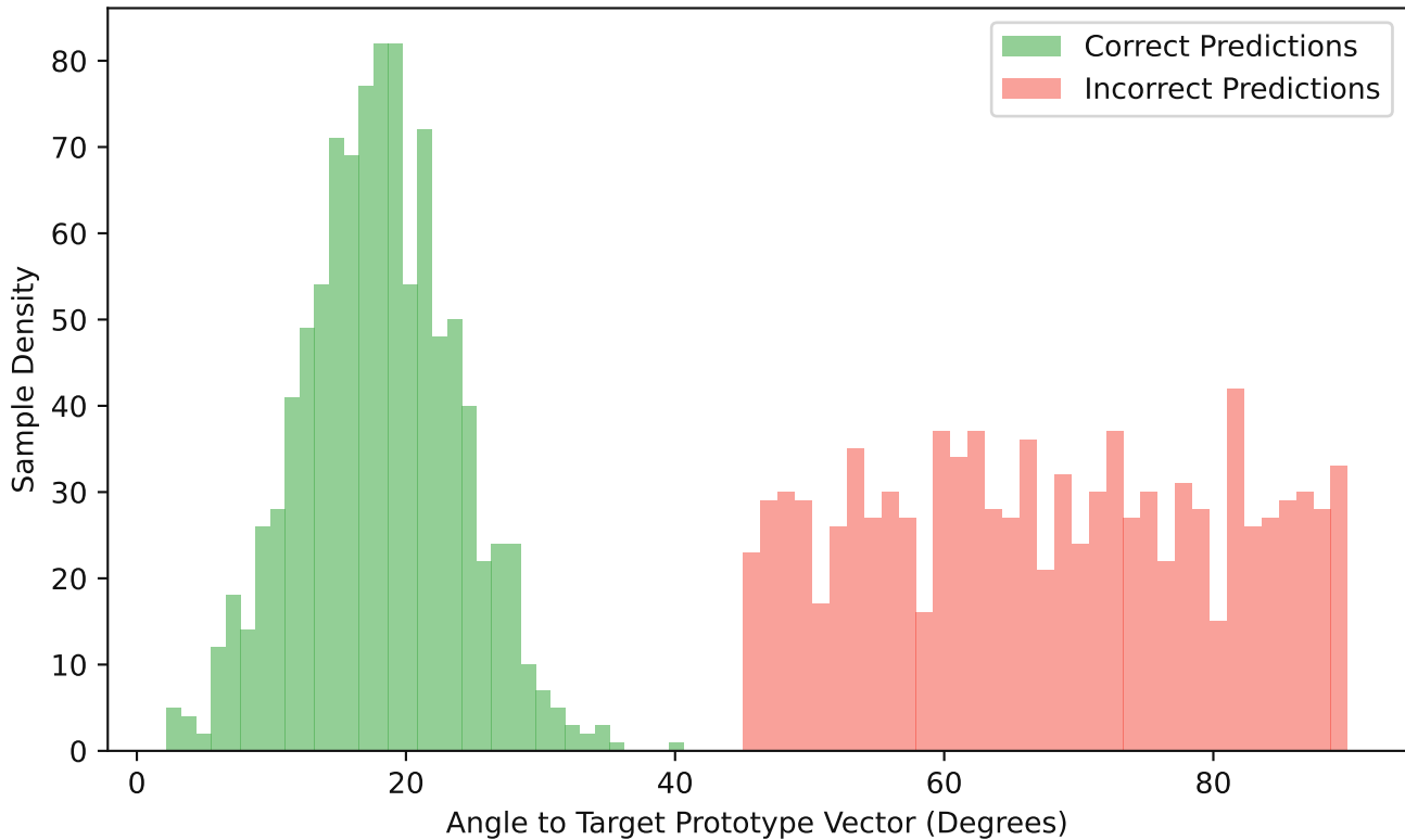
Angular Margin Distribution: Feature-to-Prototype Angle
