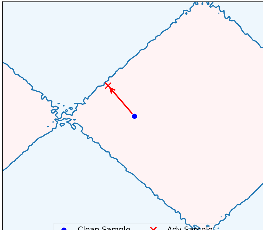
ViT-Small Decision Boundary
