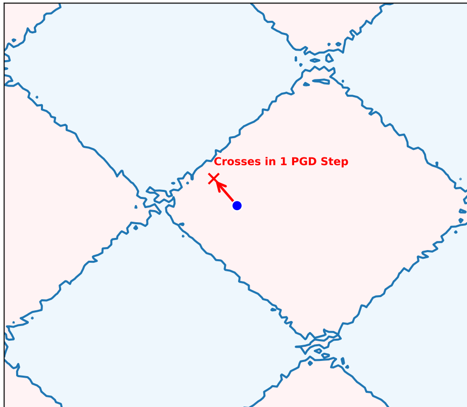
ResNet-18 Decision Boundary
