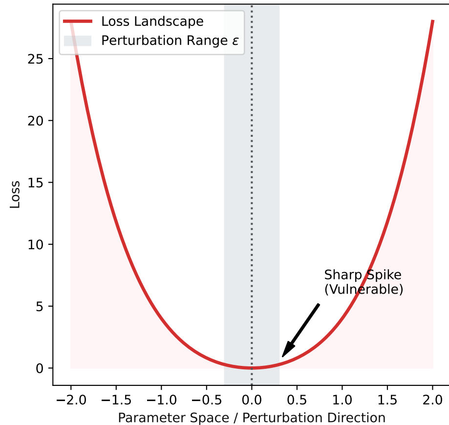
Standard CNN Landscape (Sharp Minima)
