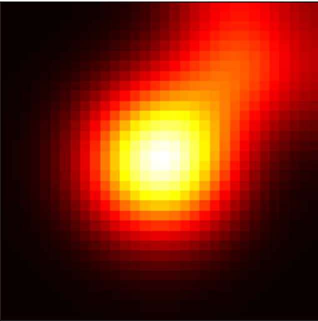
Recurrence Iteration 1
