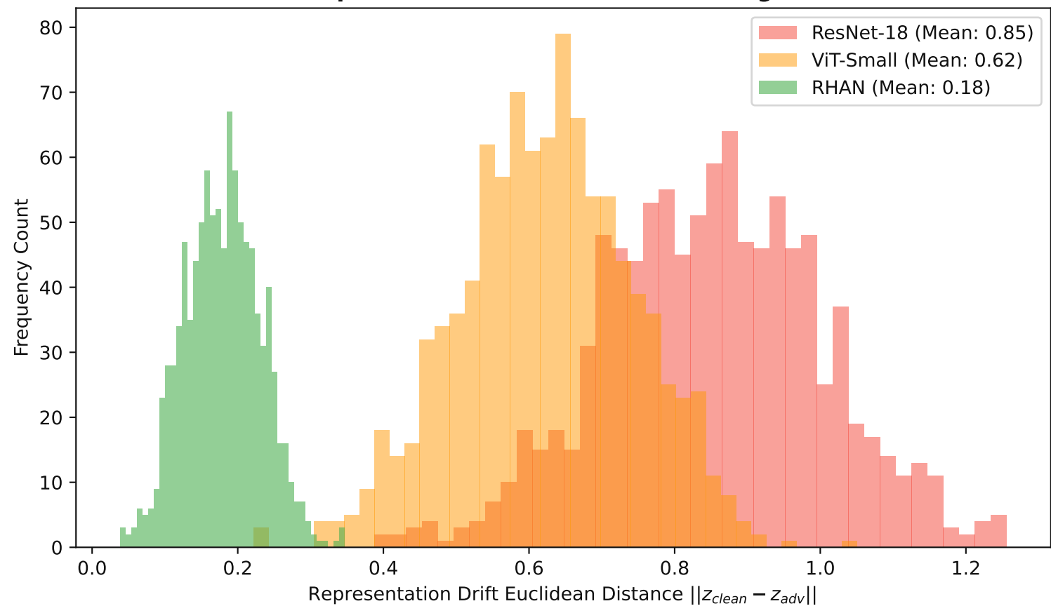
Representation Drift Distance Histogram
