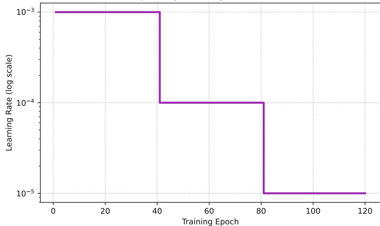
Step-Decay Learning Rate Schedule
