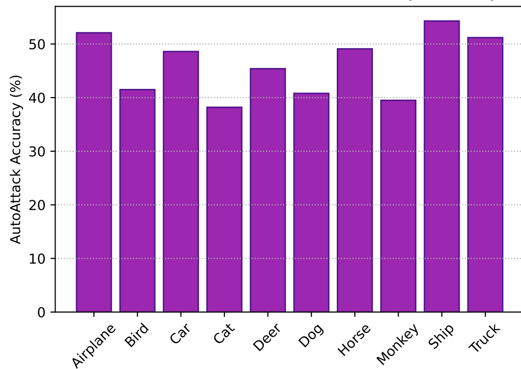
Class-wise AutoAttack Robustness (e=0.031)
