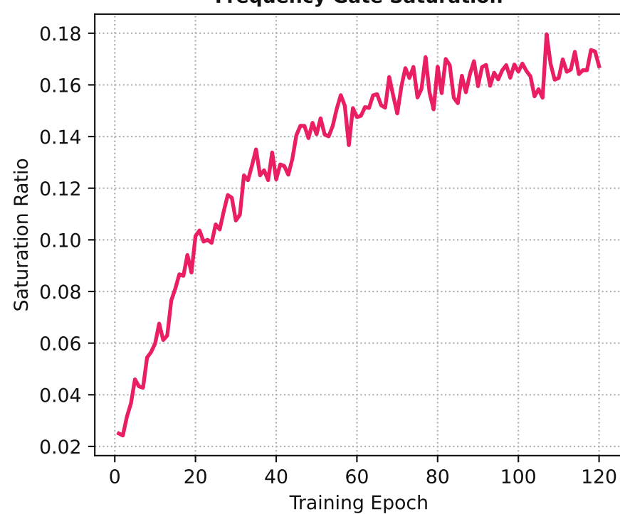
Frequency Gate Saturation
