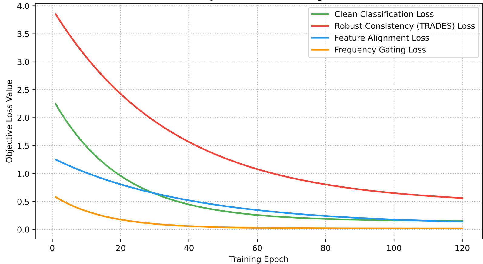
RHAN Multi-Objective Loss Convergence Profile
