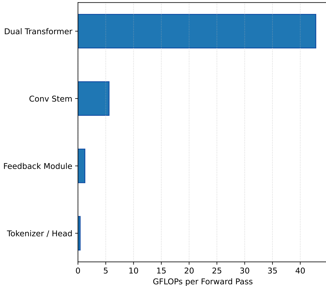
GFLOPs Distribution per Module
