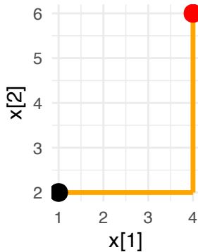
Hamming Distance
