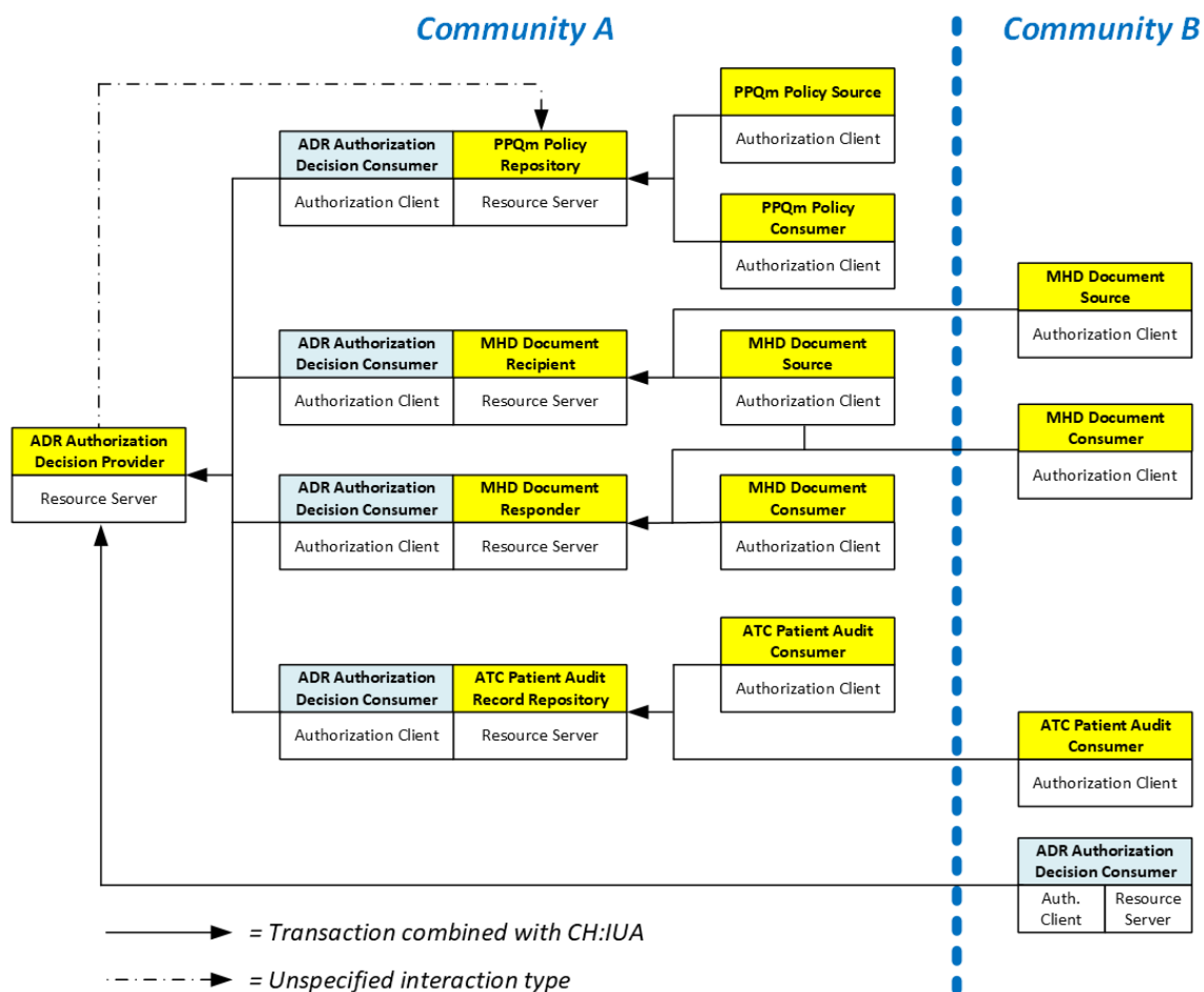
Figure 3: Actors using IUA and CH:ADR to access to sensitive data
