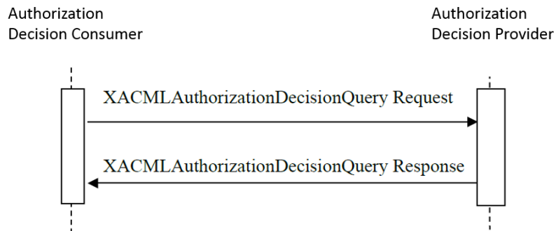
Figure 5: Sequence diagram of the CH:ADR transaction of the CH:ADR profile
