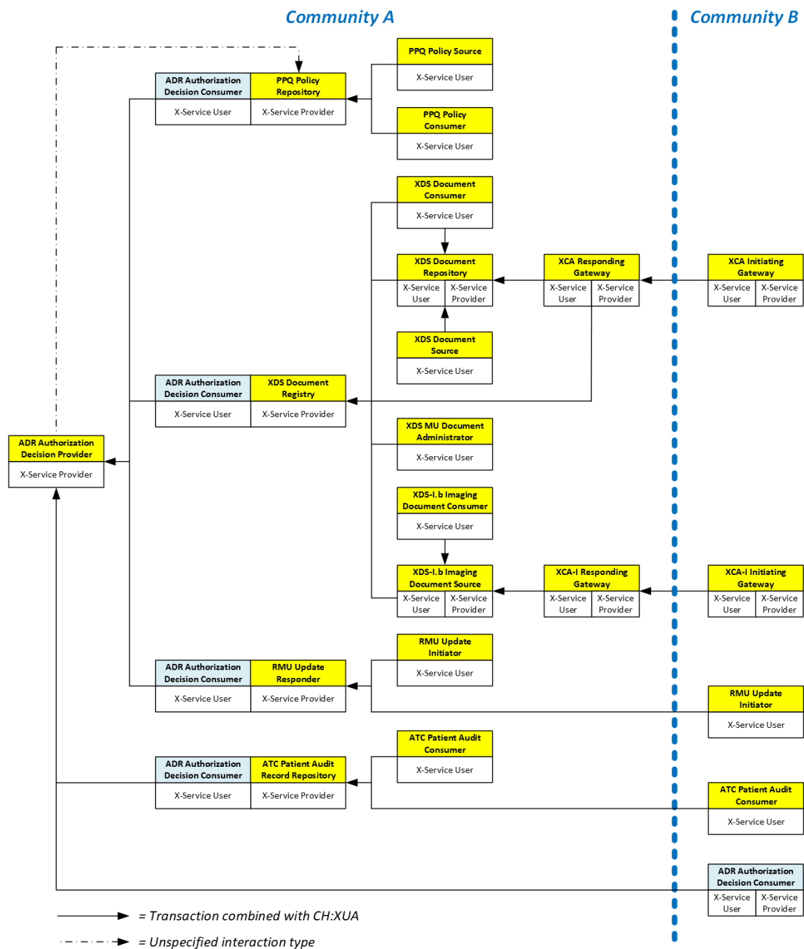
Figure 2: Actors using XUA and CH:ADR to restrict access to sensitive data
