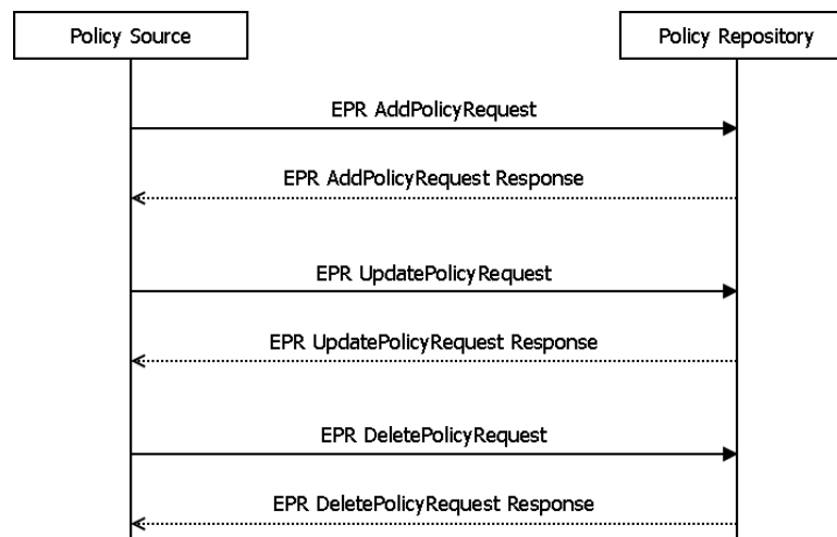
Figure 6: Sequence diagrams for the Privacy Policy Feed [CH:PPQ-1] transaction
