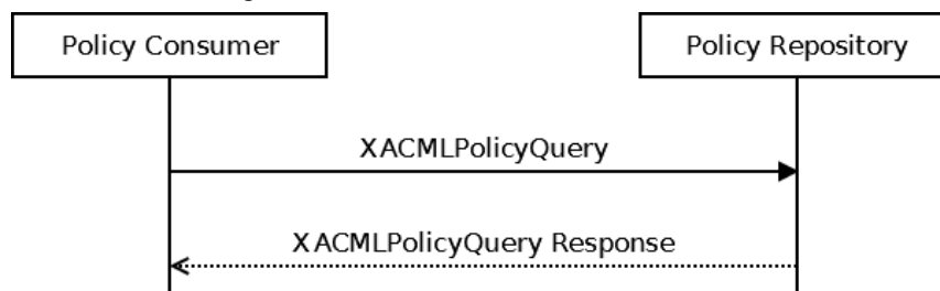
Figure 7: Sequence diagrams for the Privacy Policy Retrieve [CH:PPQ-2] transaction
