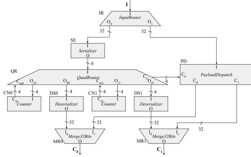
Figure 6.5: Decomposition of the MulticastUnit into separate route-parsing and payload-dispatch datapaths. The InputRouter selects the active datapath, while the route-parsing path serializes the incoming route, distributes its nibbles through the QuadRouter , accumulates the next-level counters, and reconstructs the child sub-routes through the Deserializers. For clarity, the diagram shows the simplified two-child configuration rather than the four-child structure used in the complete implementation.
