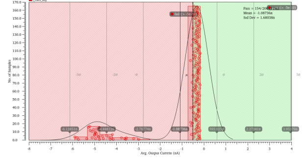
Fig. 16: Post-layout Monte Carlo simulation for mismatch and process variations
