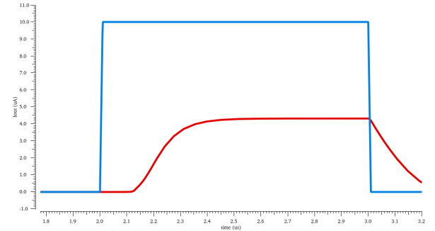
Fig. 4: Output of the DPI circuit vs. square wave input current over time
