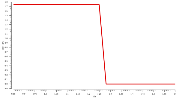
Fig. 2: Output of the sigmoid circuit vs. DC input voltage
