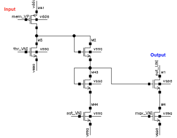
Fig. 3: Schematic of the sigmoid circuit
