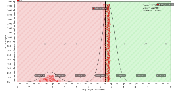
Fig. 12: Pre-layout Monte Carlo simulation for mismatch and process variations
