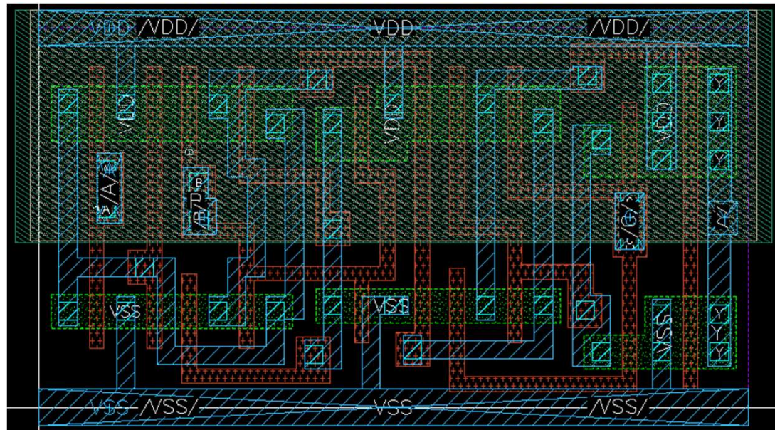
XNOR3X2 layout
