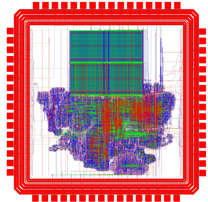
Final layout
