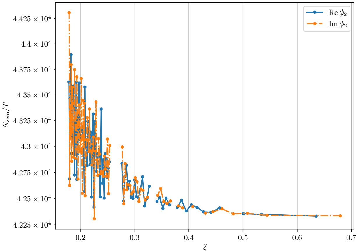
Number of transitions per quasi-period for \psi_2
