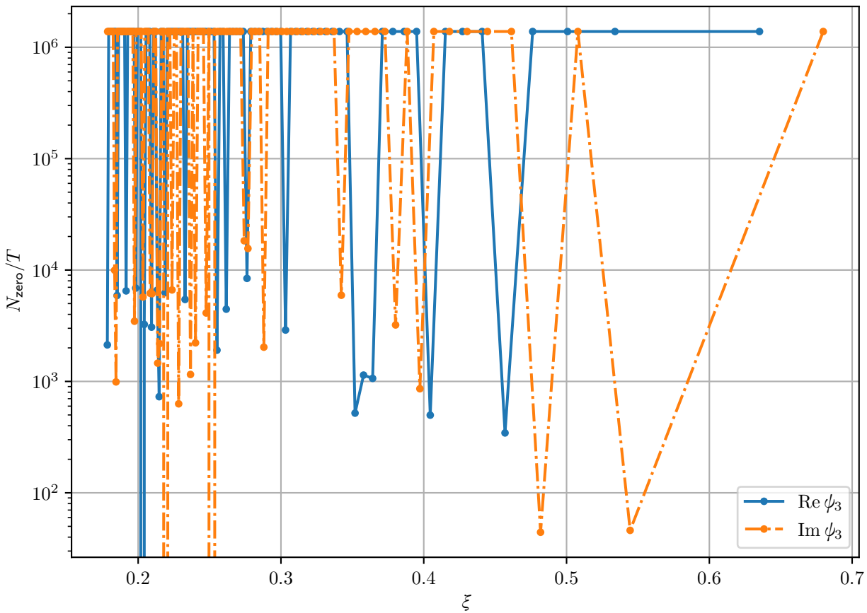
Number of transitions per quasi-period for \psi_3
