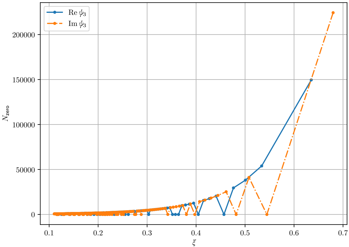
Number of zero transitions for \psi_3
