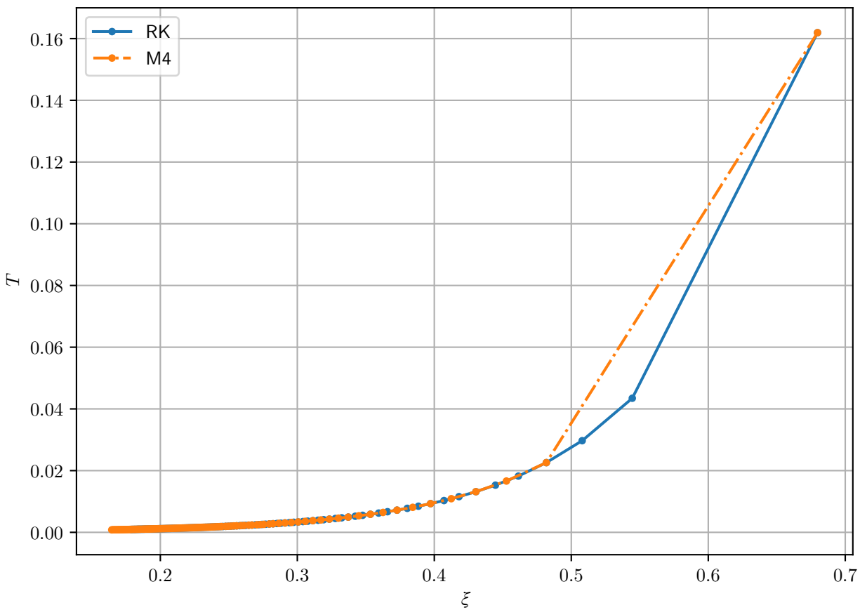
Quasi-period of \text{Im } \psi_1 , different methods
