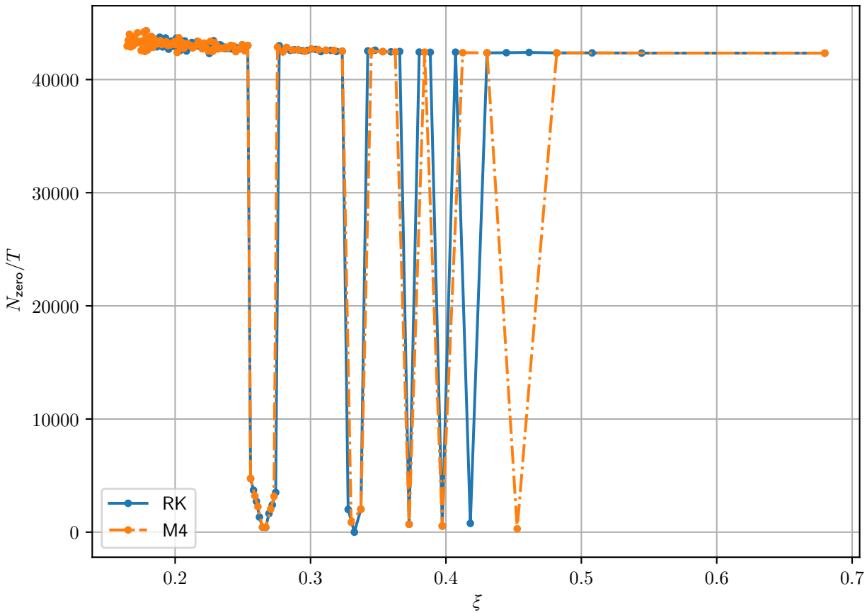
Number of transitions per quasi-period for \text{Im } \psi_2 , different methods
