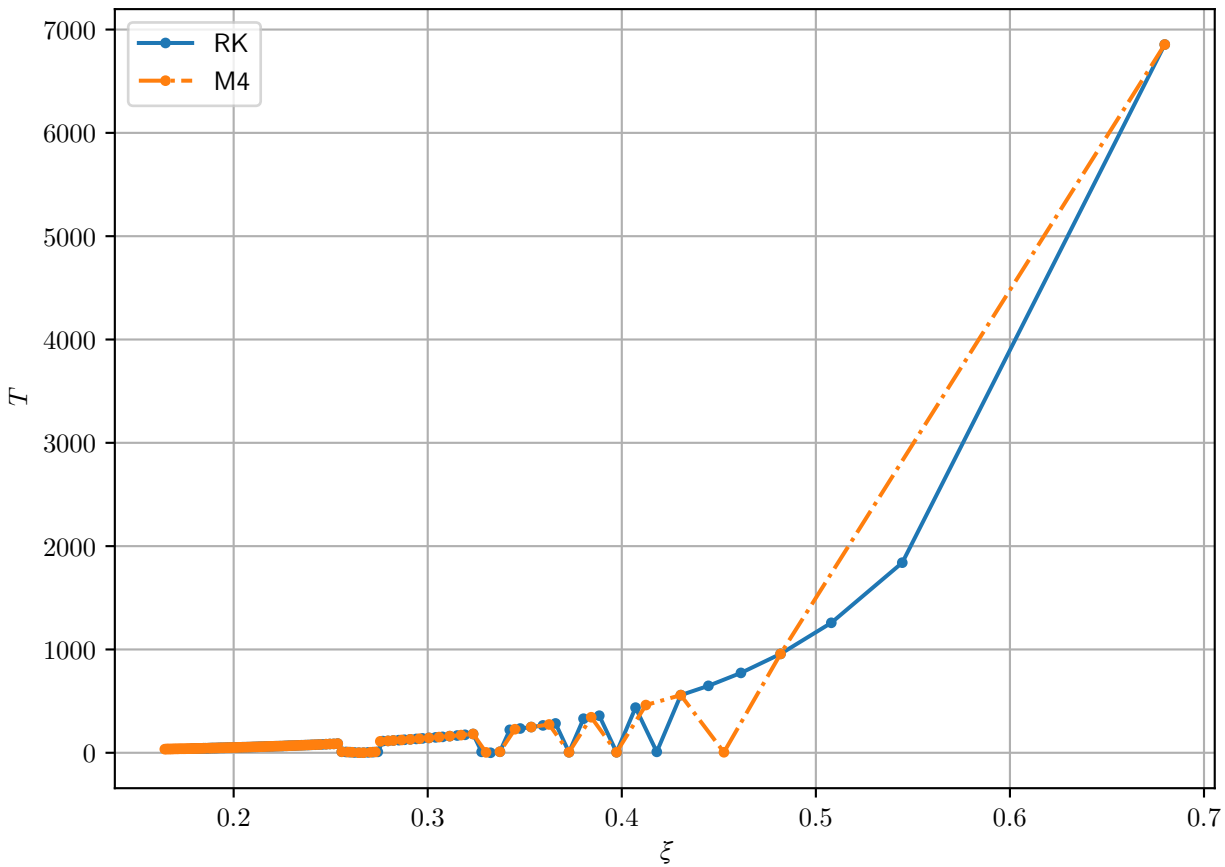
Quasi-period of \text{Im } \psi_2 , different methods
