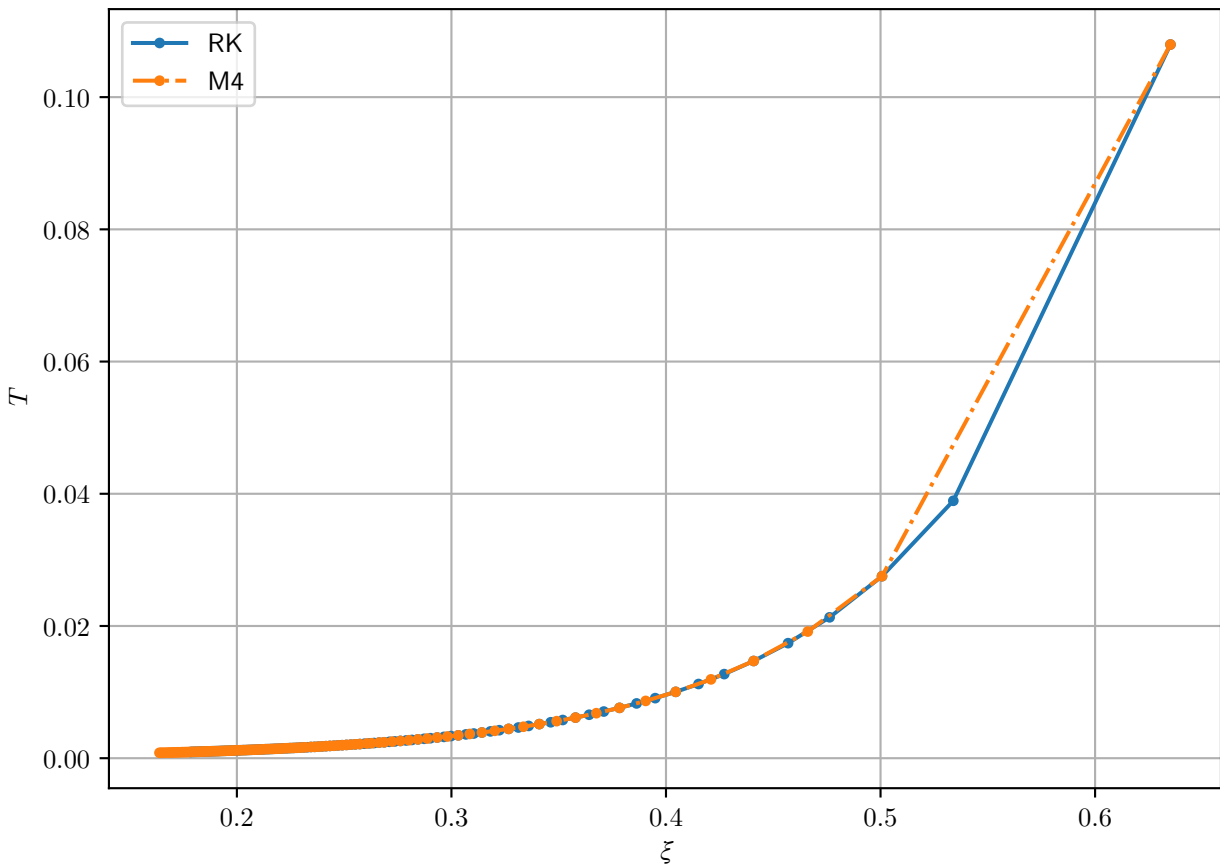
Quasi-period of \text{Re } \psi_1 , different methods
