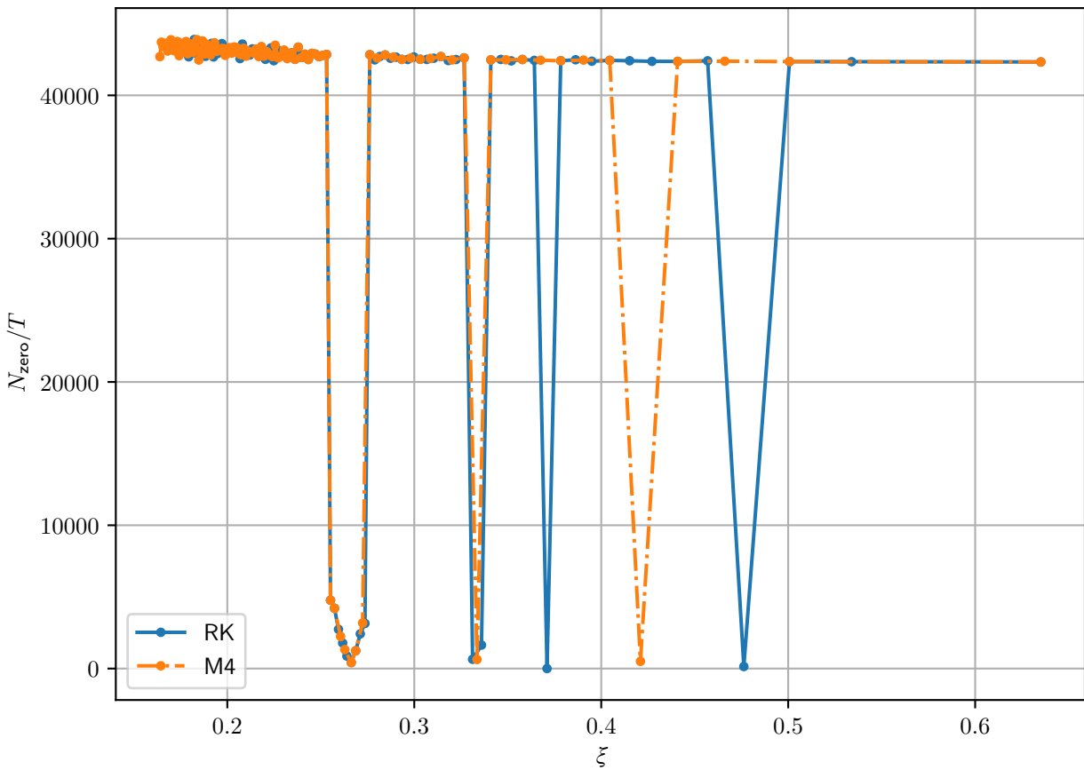
Number of transitions per quasi-period for \text{Re } \psi_2 , different methods
