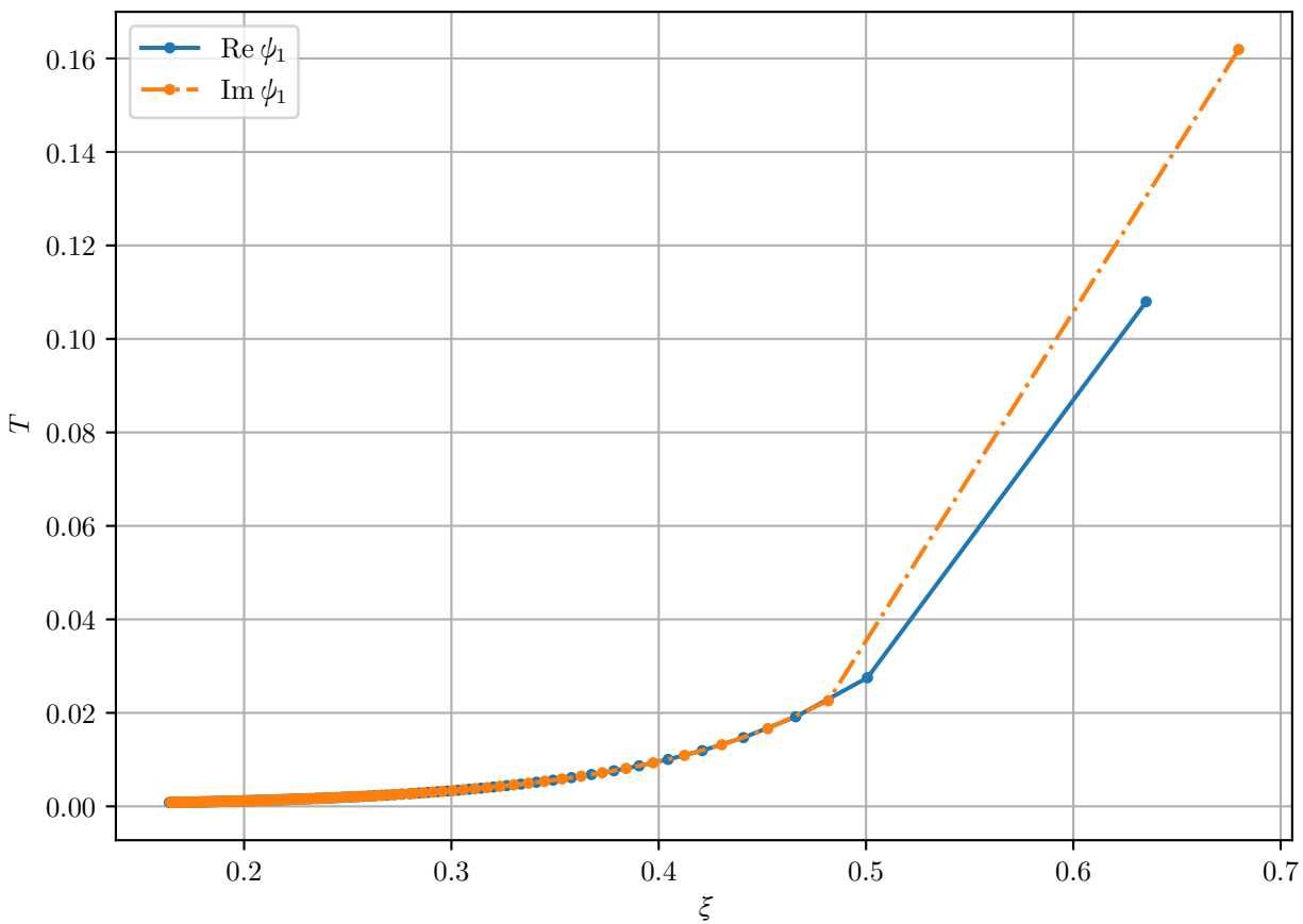
Quasi-period of \psi_1
