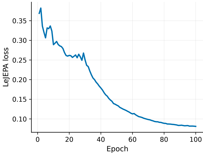
(a) LeJEPA pretraining (final=0.0811)
