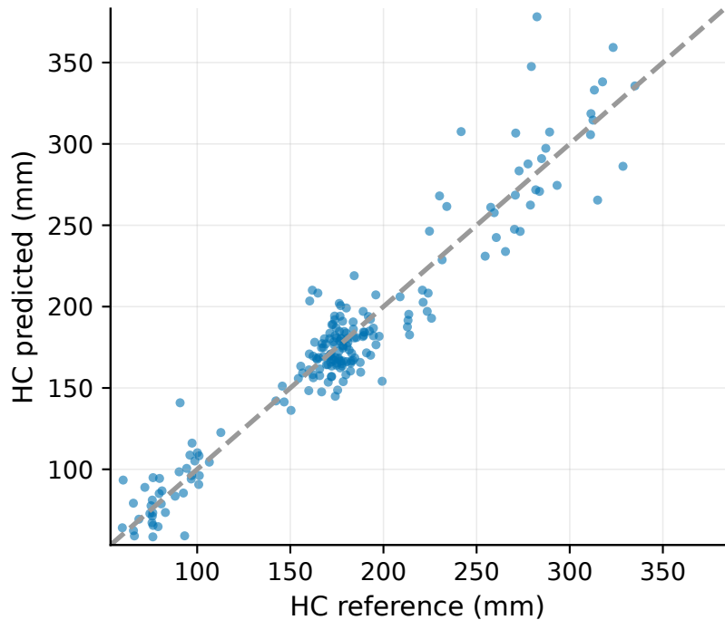
(a) Correlation ( r=0.955 , MAE=13.48 mm)
