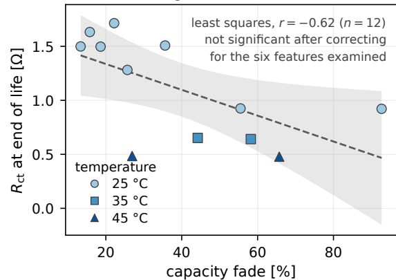
(a) end-of-life charge-transfer resistance vs fade
