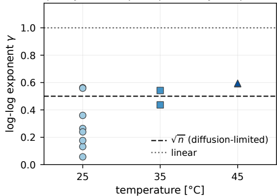
(b) capacity-loss shape exponent by temperature
