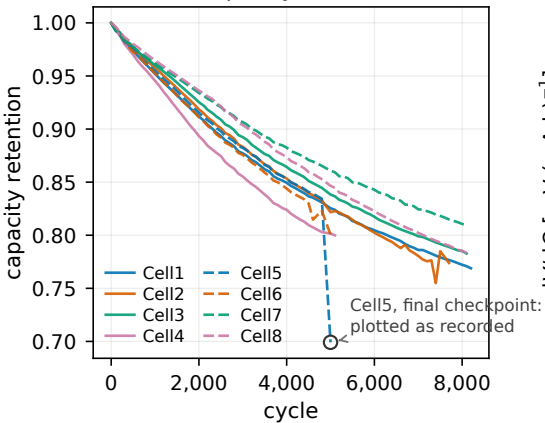
(a) measured capacity retention (8 cells)
