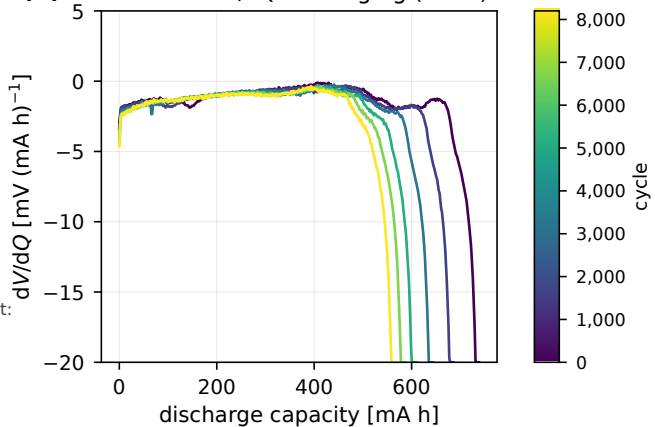
(b) low-rate dV/dQ over aging (Cell1)
