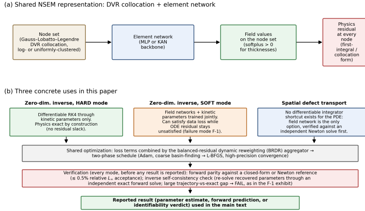
Fig. 9 NSEM workflow. (a) Shared representation: field values on a discrete-variational-representation collocation node set produced by an element network (MLP or KAN backbone), with physics residuals enforced at every node. (b) The three configurations used in this work, the shared two-phase optimization, and the verification step each configuration passes before its results are reported.
