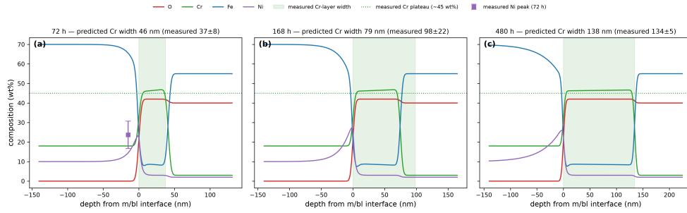
Fig. 6 Zero-free-parameter composition-map prediction against Veile et al.’s measured EDX features at (a) 72, (b) 168, and (c) 480 h. Curves are predicted composition profiles (O, Cr, Fe, Ni; weight percent) versus depth from the metal/barrier-layer interface; overlays mark the measured features compared: Cr-layer width (shaded band), Cr plateau level (~45 wt%, dotted), and the 72-h Ni-peak amplitude ( 23.7 \pm 7.0 wt%, error bar). Full digitized EDX traces are not available, so the comparison is feature-based.
