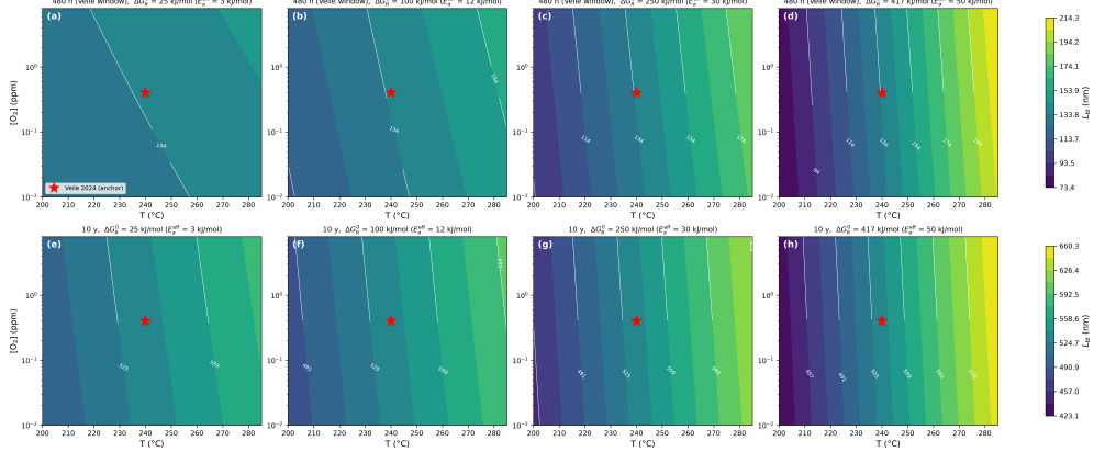
Fig. 8 Operating-envelope sensitivity maps: predicted L_{bl} at (a–d) 480 h and (e–h) ten years over the scanned envelope (200–285°C, 0.01–8 ppm O_2 ), for \Delta G_R^0 = 25, 100, 250 and 417 kJ/mol—effective activation energies \alpha_3 \Delta G_R^0 of 3, 12, 30 and 50 kJ/mol, spanning the full plausible range rather than only the low values a transferred supercritical-water transfer coefficient implies. The marker locates the Veile et al. calibration condition. Each row shares a common color scale, so the widening spread from left to right is the sensitivity increasing with activation energy.
