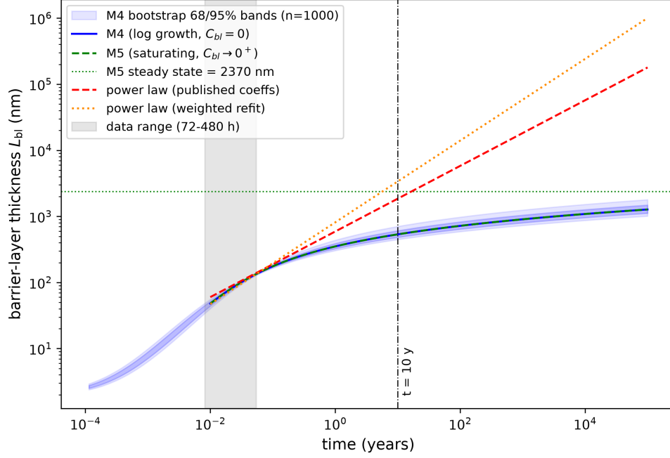
Fig. 7 Long-time prediction with propagated parametric uncertainty: M4 (logarithmic growth) versus M5 (saturating branch) versus the two power-law variants, to 10^5 years. Shaded bands are the 68% and 95% intervals of the 1000-member parametric bootstrap propagated through the M4 closed form, conditional on the M4 model structure and the reported standard errors; the M5 curve is indistinguishable from M4 at all feasible exposures. The vertical line marks the ten-year horizon.
