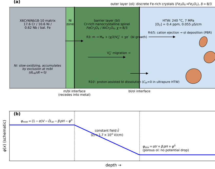
Fig. 1 Duplex-oxide model schematic. (a) Layer structure (metal | Ni enrichment zone | Cr-rich nanocrystalline spinel barrier layer | Fe-rich outer-layer crystals | hydrothermal water) and the retained interfacial reactions. (b) Potential distribution across the duplex oxide under the constant-field assumption. Reaction labels and potential-drop symbols follow the SI derivation.
