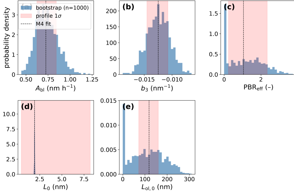
Fig. 4 Bootstrap ensemble versus profile likelihood: 1000-member parametric bootstrap distribution for each M4 parameter, compared against the profile-likelihood 1\sigma band.
