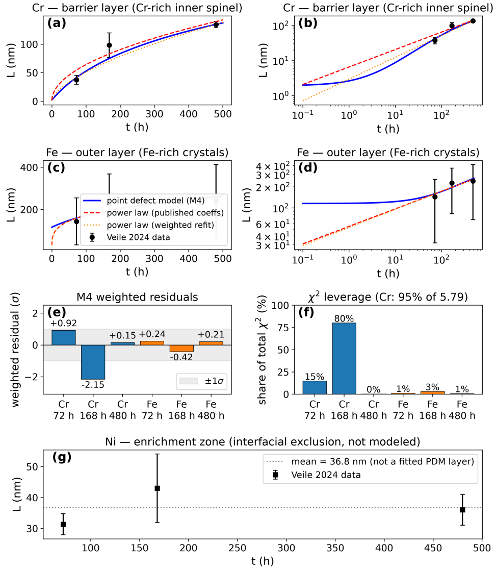
Fig. 2 M4 fit and the empirical power law against the measured layer-thickness data. (a, b) Cr barrier layer, linear and log-log axes; (c, d) Fe outer layer, linear and log-log axes. Points with error bars are the means \pm standard deviations of Table 1 (the fits weight residuals by standard errors, SD/\sqrt{n} ); curves are the M4 mechanistic fit and the two power-law variants (published coefficients and weighted refit). (e) Weighted residuals of the M4 fit at the six data points, and (f) each point's share of the total \chi^2 : the chromium layer carries 95% of the fit statistic and the 168 h chromium point alone 80%, with the +, -, + chromium residual pattern indicating a systematic curvature miss rather than scatter (Table 3). (g) Ni enrichment-zone thickness, shown for completeness with its measured mean (dotted); as in Veile et al.'s own analysis, this zone is not a growing PDM layer, and its dedicated transport fit appears in Section 2.6.
