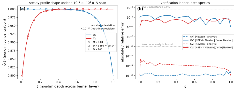
Fig. 5 Steady spatial solve. (a) Steady-state nondimensional profile shape with diffusivity scaled by 0.01 \times to 100 \times ; the curves coincide to machine precision, confirming the diffusivity-cancellation result. (b) Verification ladder: Newton versus analytic, and NSEM versus Newton, for both defect species; horizontal lines mark the 10^{-10} and 0.5% acceptance bounds.
