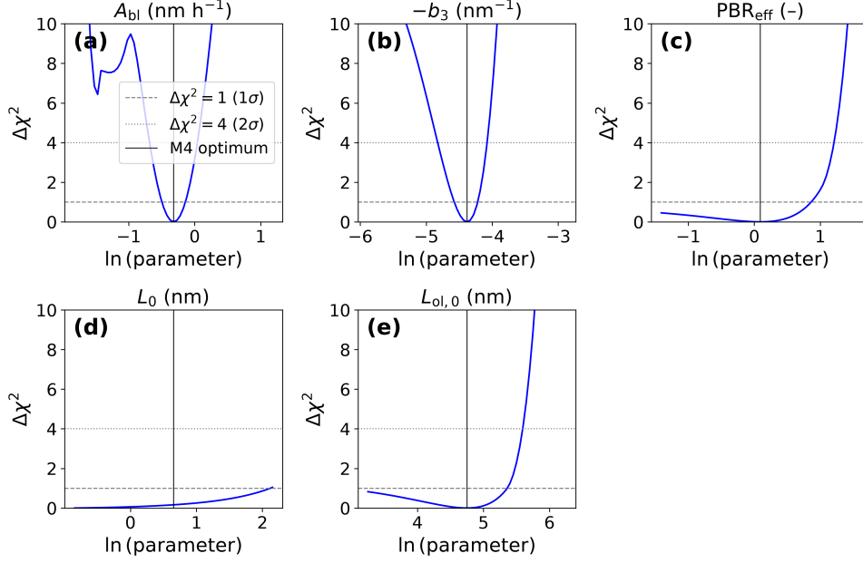
Fig. 3 Profile-likelihood identifiability map: \Delta\chi^2 over the data residuals versus each M4 parameter (natural-log abscissa), with the 1\sigma ( \Delta\chi^2 = 1 ) and 2\sigma ( \Delta\chi^2 = 4 ) thresholds marked.
