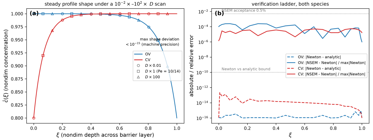
Figure 6: Steady spatial solve. (a) Steady-state nondimensional profile shape with diffusivity scaled by 0.01\times to 100\times ; the curves coincide to machine precision, confirming the diffusivity-cancellation result. (b) Verification ladder: Newton versus analytic, and NSEM versus Newton, for both defect species; horizontal lines mark the 10^{-10} and 0.5% acceptance bounds.
