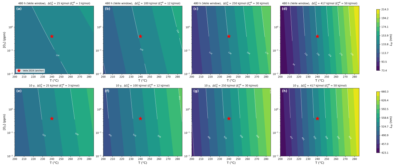
Figure 9: Operating-envelope sensitivity maps: predicted L_{b1} at (a–d) 480 h and (e–h) ten years over the scanned envelope (200–285°C, 0.01–8 ppm O_2 ), for \Delta G_R^0 = 25, 100, 250 and 417 kJ/mol—effective activation energies \alpha_3 \Delta G_R^0 of 3, 12, 30 and 50 kJ/mol, spanning the full plausible range rather than only the low values a transferred supercritical-water transfer coefficient implies. The marker locates the Veile et al. calibration condition. Each row shares a common color scale, so the widening spread from left to right is the sensitivity increasing with activation energy.
